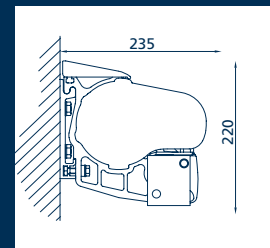
Montaggio a parete Wall installation
