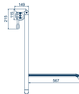
Vista con ingombri laterali - View with lateral encumbrances
