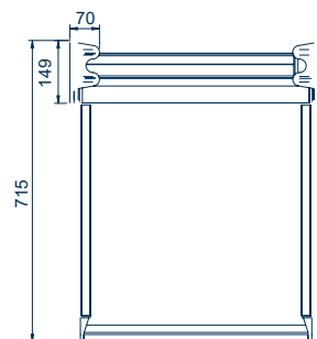
Pianta - Face view
